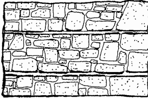
D. Coursed random rubble
